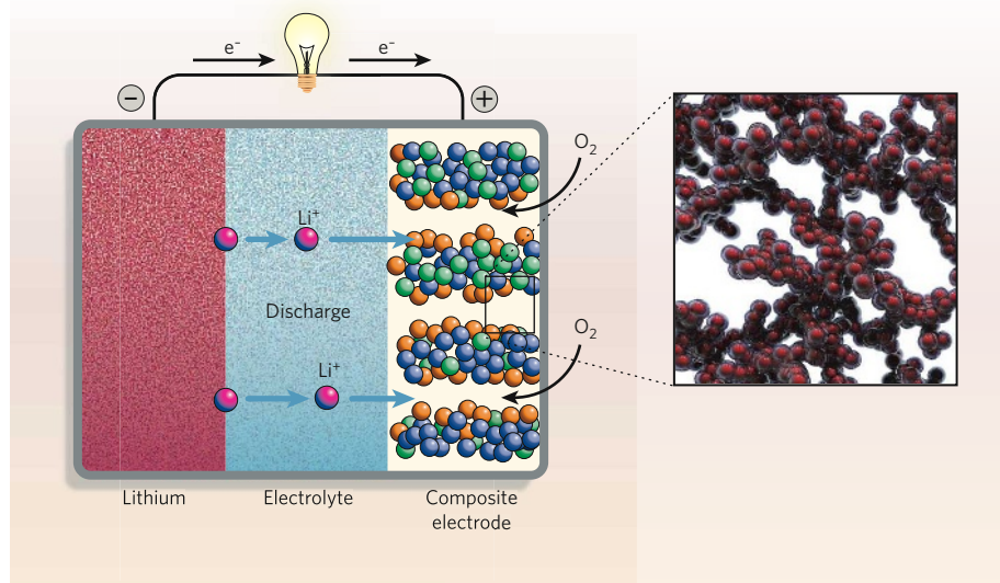
Figure 5 | Lithium-air batteries. Left, the mechanism used in lithium-air batteries (courtesy of A. Debard et al. , Univ. St Andrews). Right, three-dimensional nanostructured electrodes made from depositing 10- to 20-nm-thick layers of \text{MnO}_2 onto a carbon foam using a low-temperature process (according to ref. 20) that could be used to enhance the kinetics of the lithium-air electrode (three-dimensional schematic courtesy of J. W. Long and D. R. Rolison, US Naval Research Lab.).
